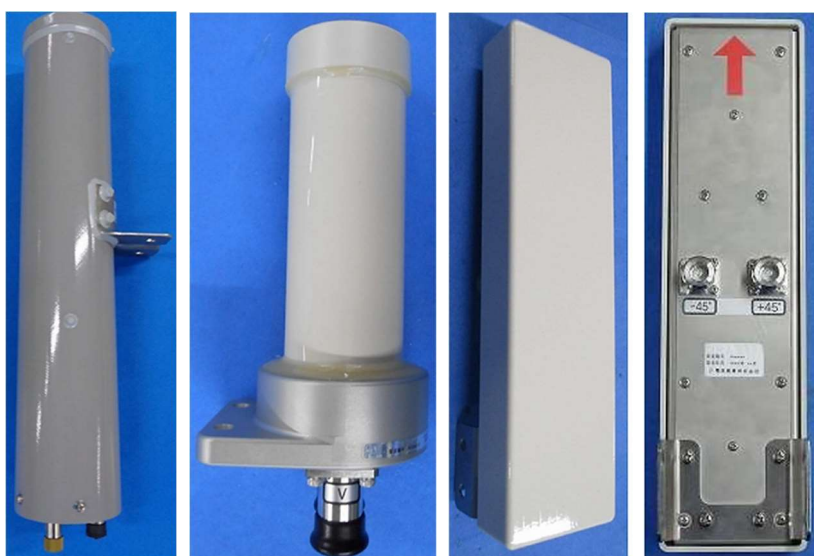
△CBRS/C-Band Antenna
