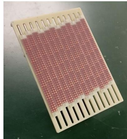
Incident Reflection Angle Variable Reflector
